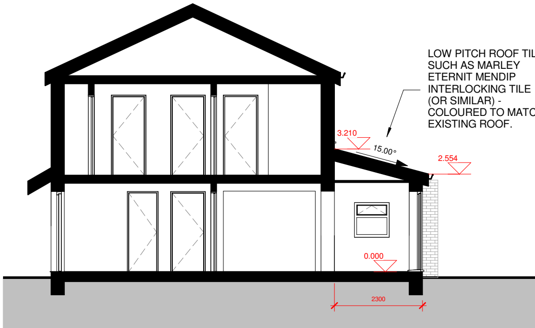
3 | P-005 PROPOSED SECTION 1 : 100
