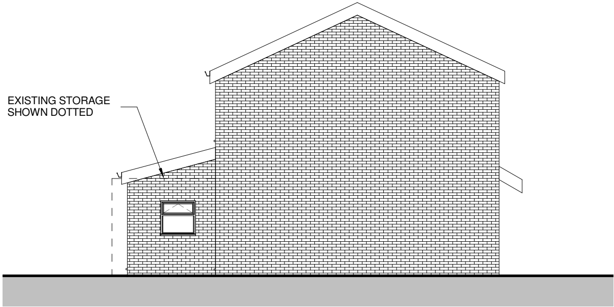
2 | P-005 PROPOSED SIDE ELEVATION 1 : 100
