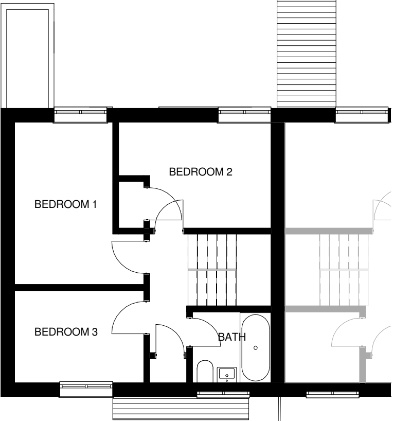
2 | P-003 EXISTING FIRST FLOOR PLAN 1 : 100
