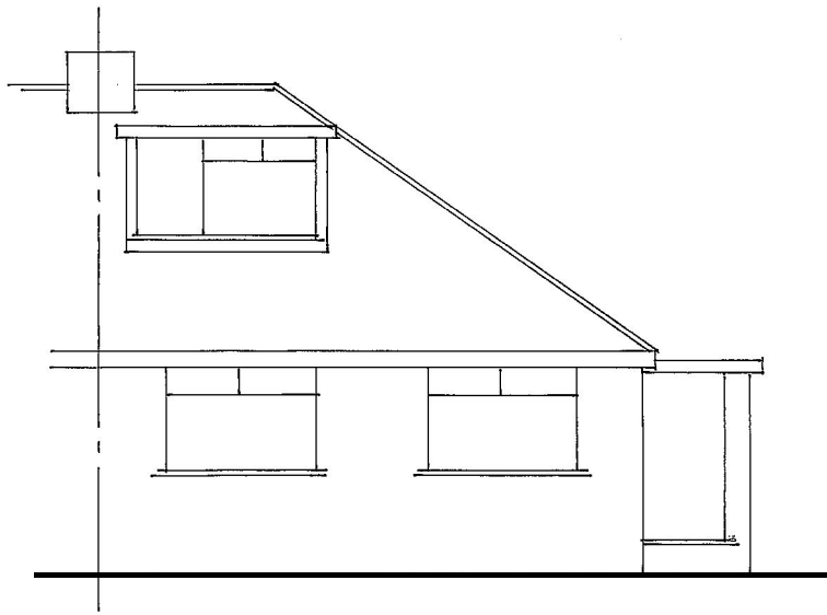
Existing NW/Front Elevation
