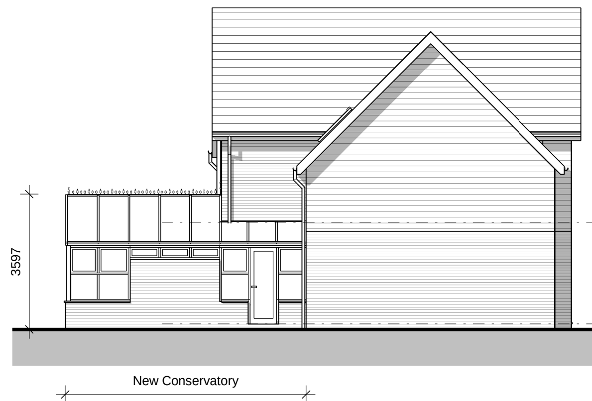
South Elevation - Proposed 1 : 100
