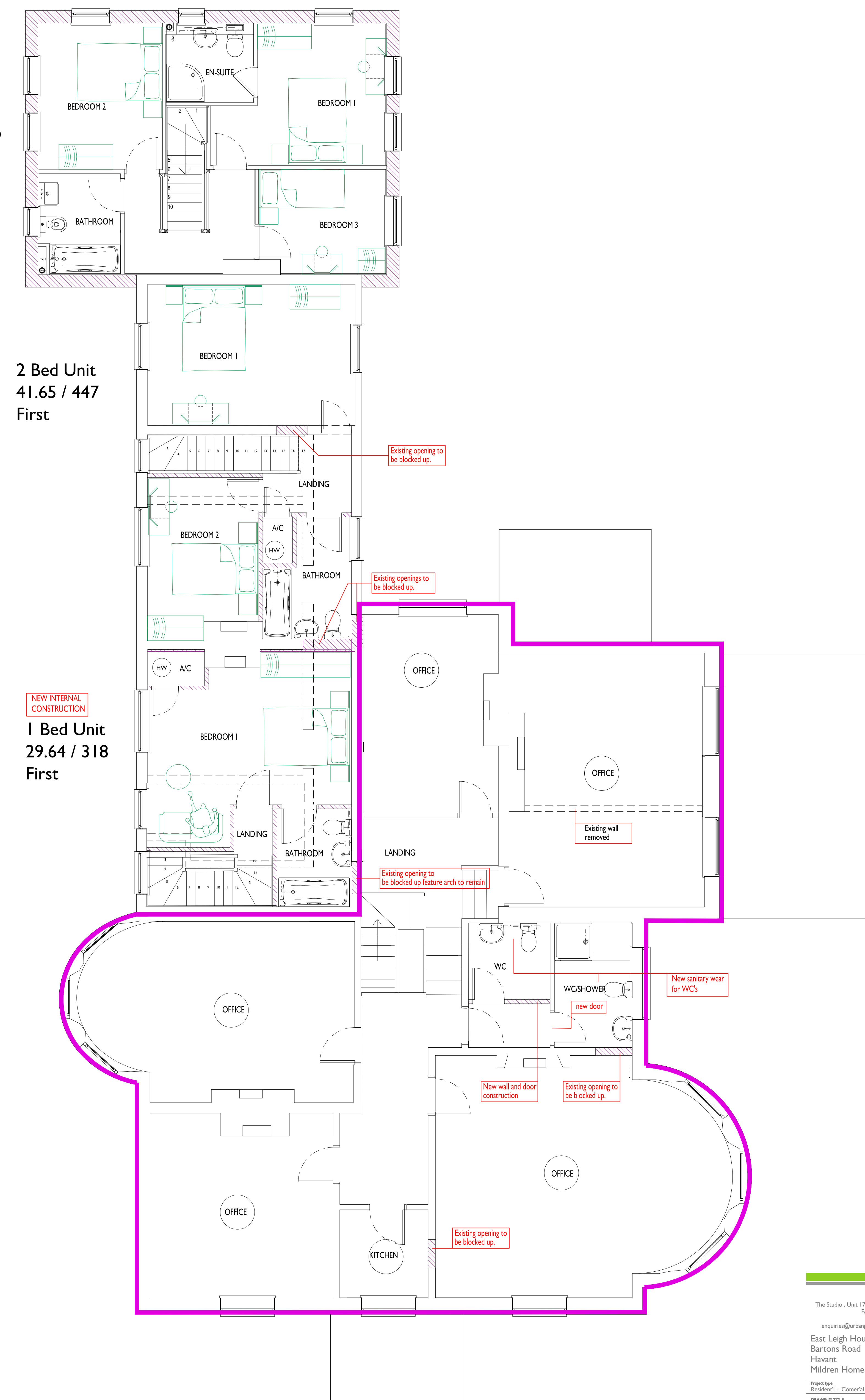
Proposed First Floor Plan
