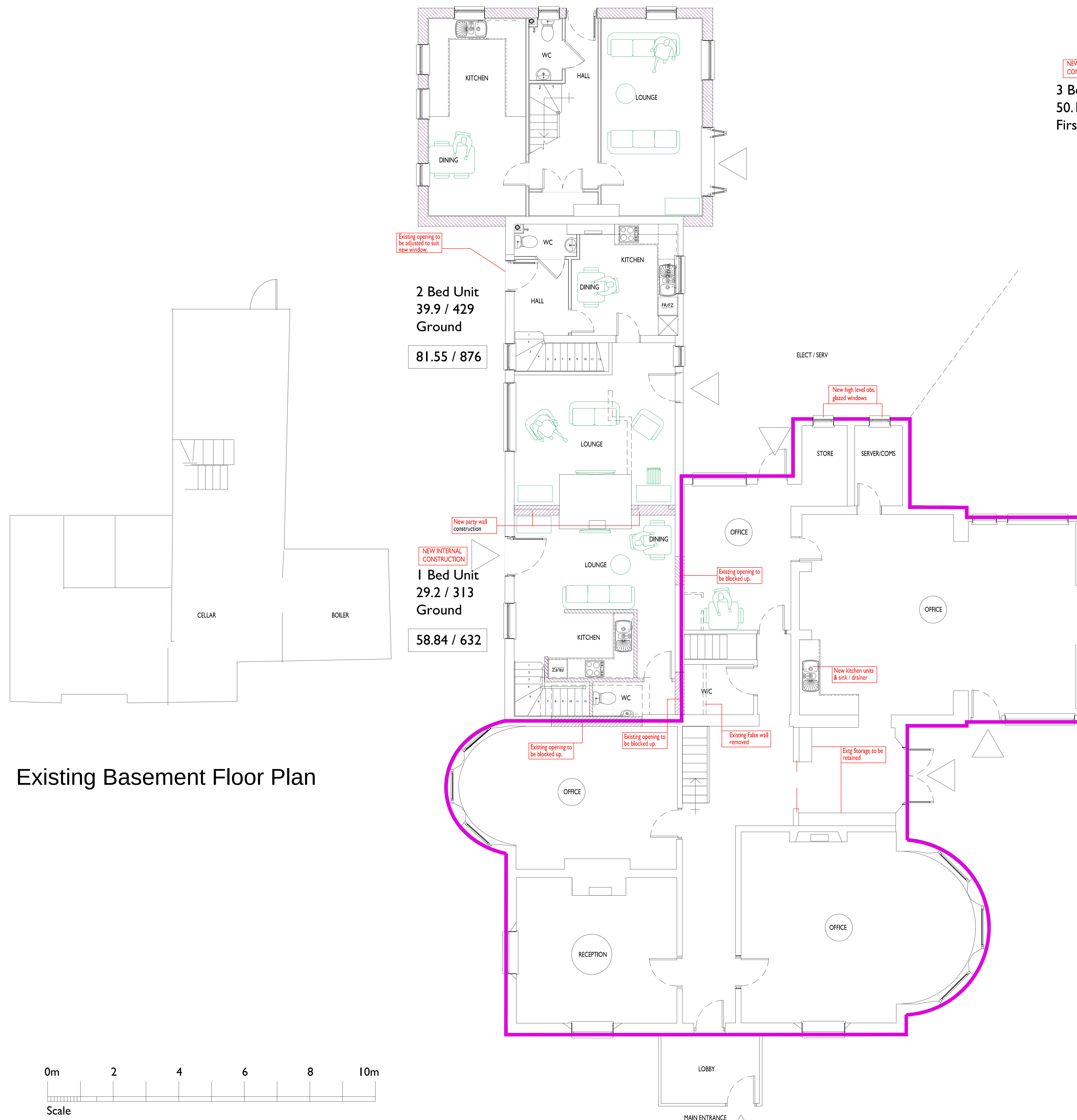
Proposed Ground Floor Plan
