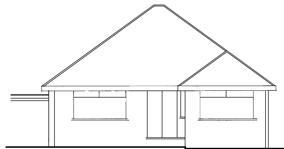
Existing SE/Front Elevation
