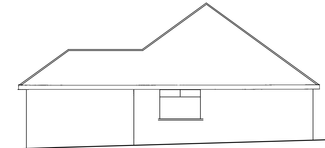
Existing NE/Side Elevation
