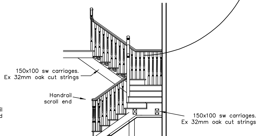
SIDE ELEVATION
