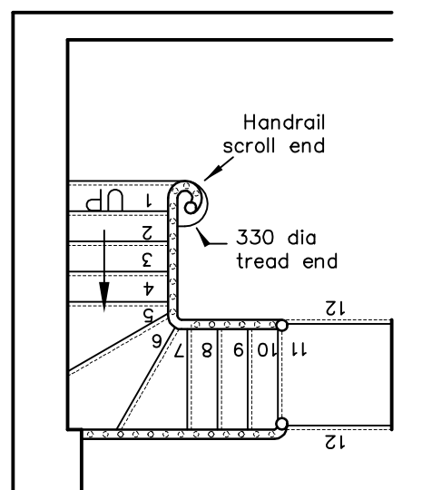
PLAN (First)
