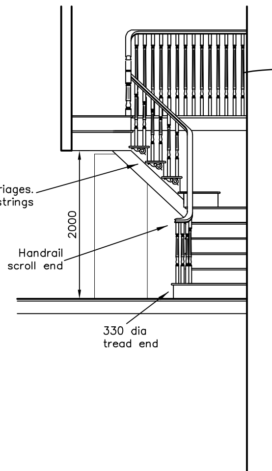
SIDE ELEVATION
