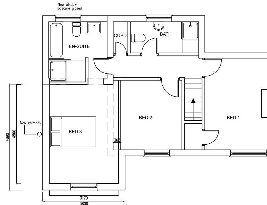
FIRST FLOOR PROPOSED
