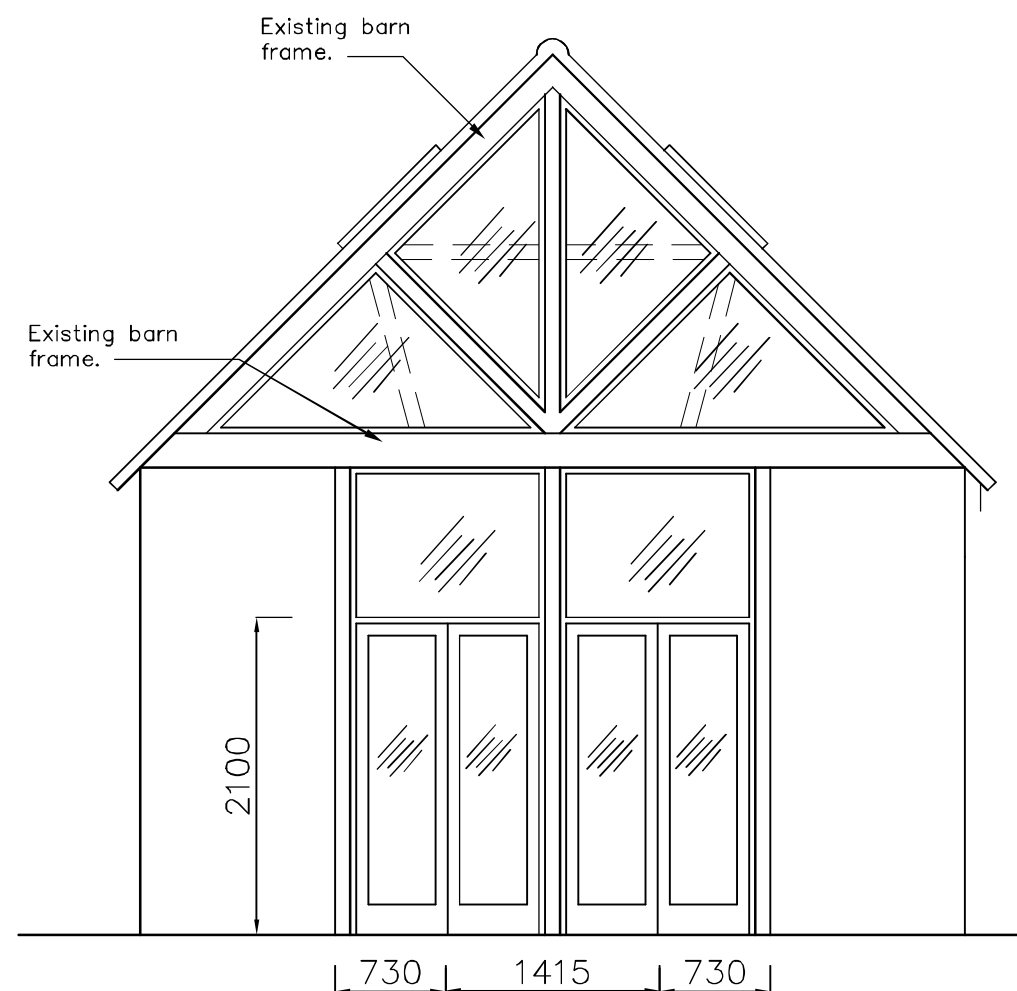
NEW DOORS AND GLAZING
