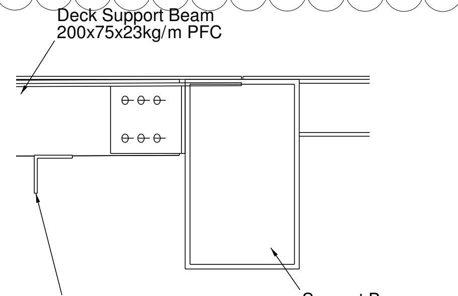
DETAIL C 1:10
