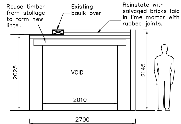
PROPOSED SOUTH
