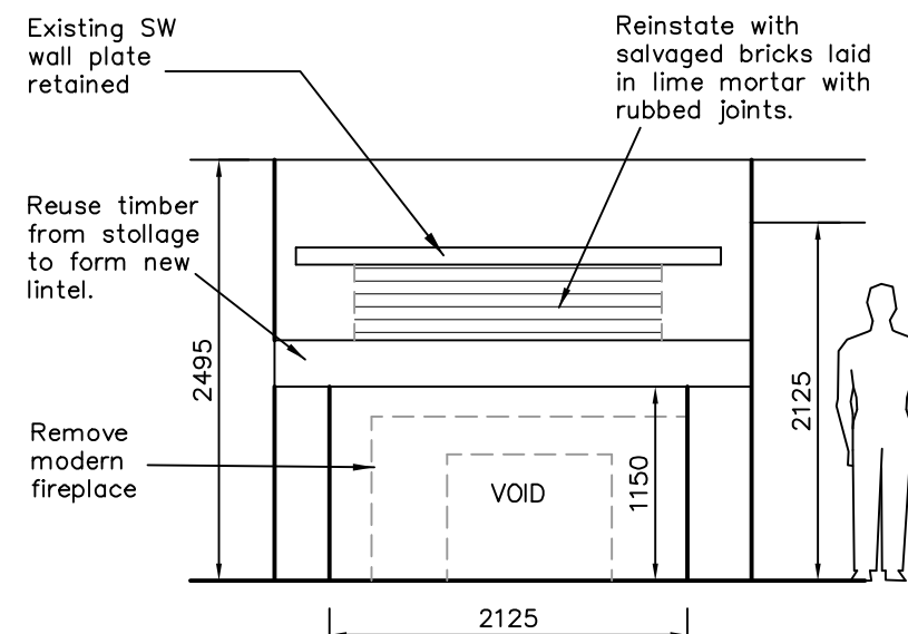
PROPOSED NORTH
