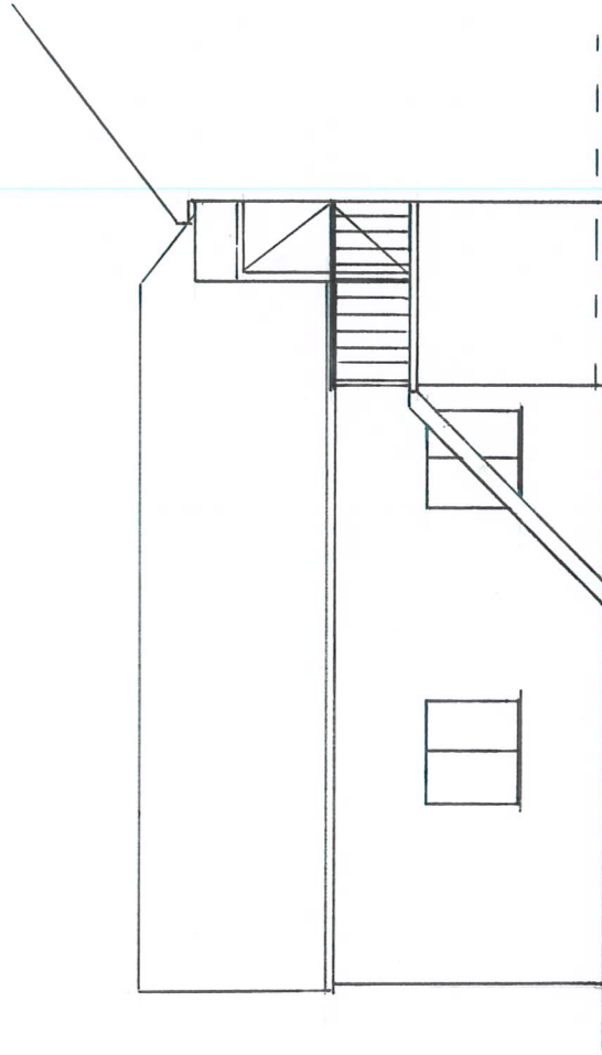
EXISTING GARAGE SIDE ELEVATION
