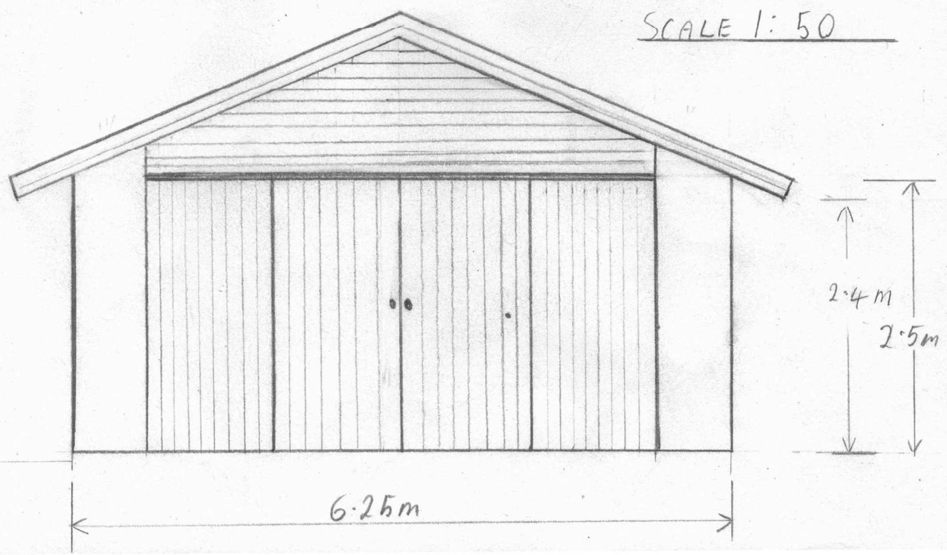
NORTH ELEVATION
