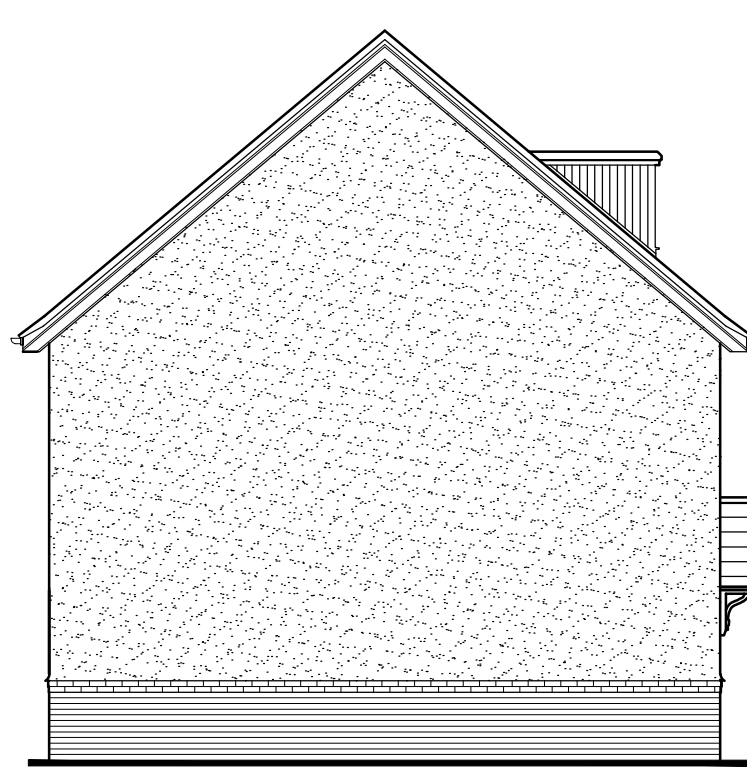
Side Elevation
