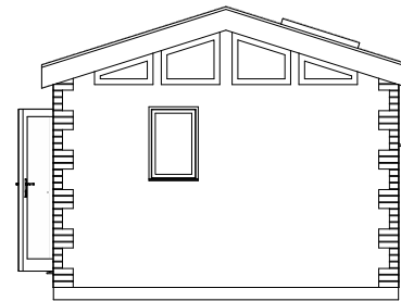
North West Elevation
