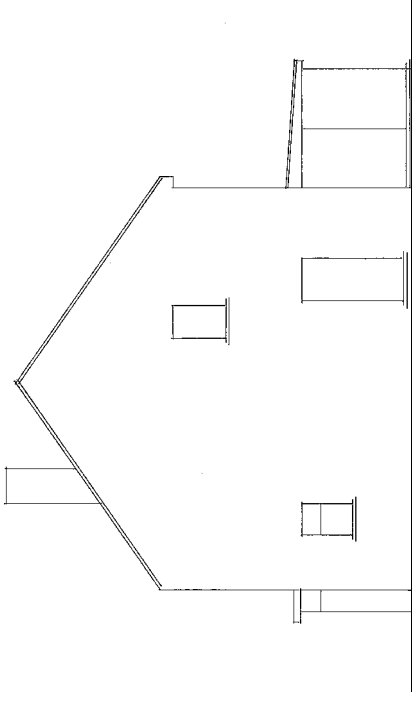
Existing SW/Side Elevation
