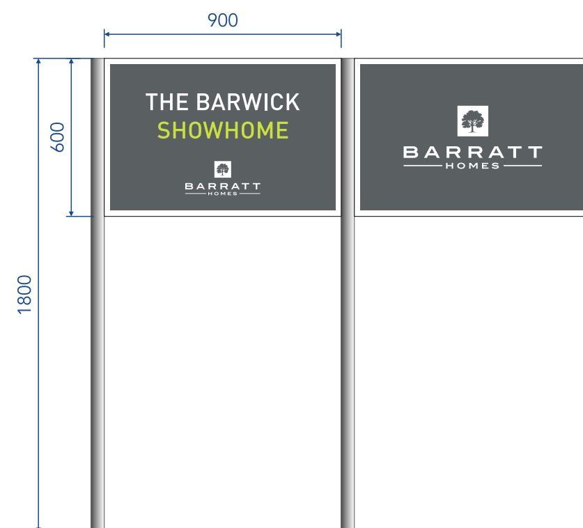
ITEM 5 Secondary Sign Standard Scale 1:20
