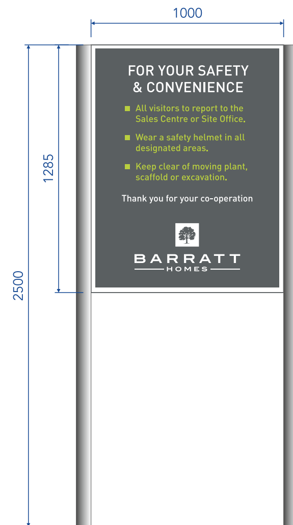
ITEM 3 Secondary Sign Medium Scale 1:20
