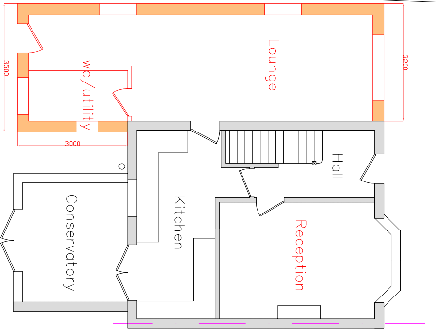
Proposed Ground Floor Layout
