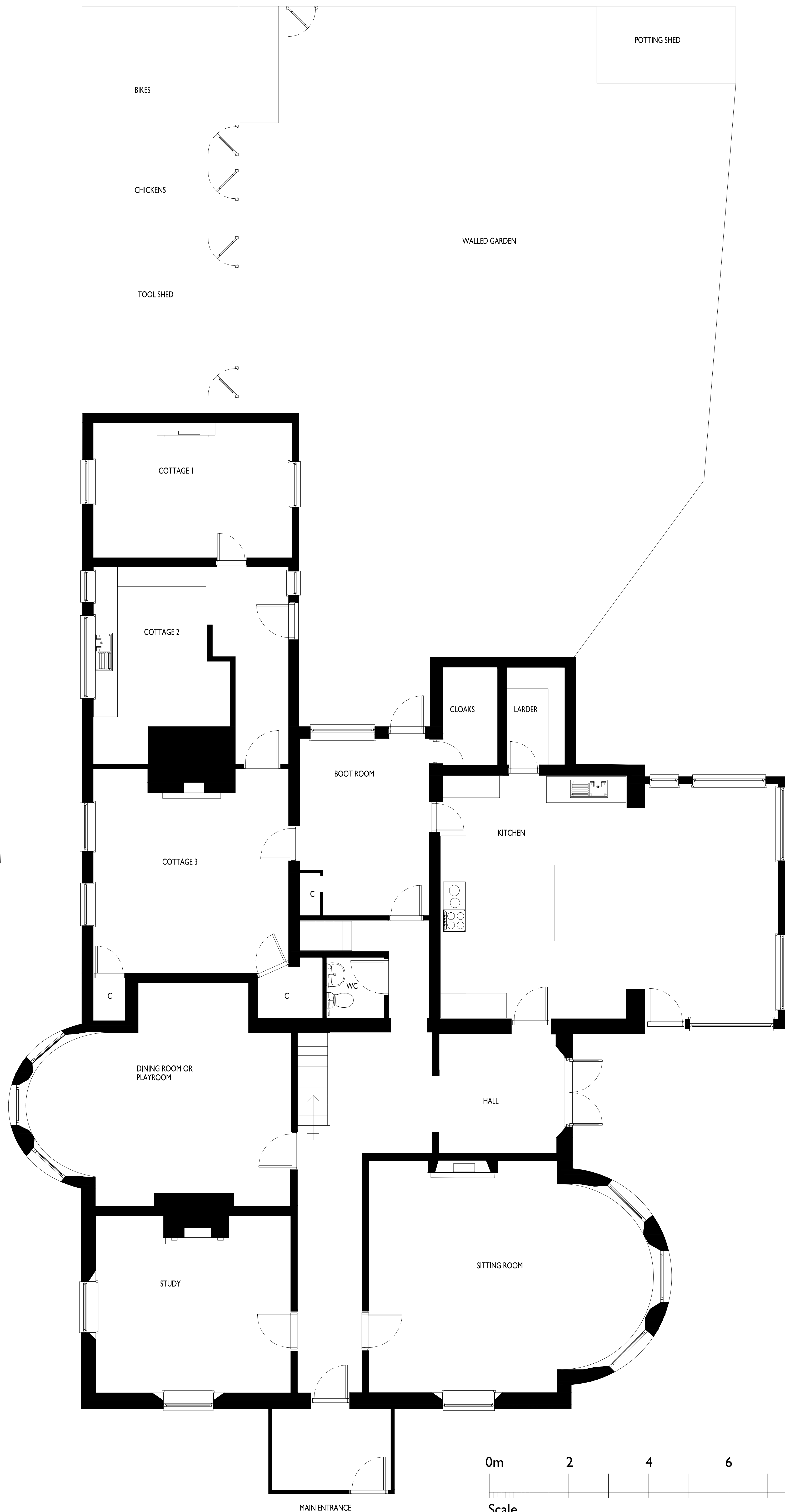
Existing Ground Floor Plan
