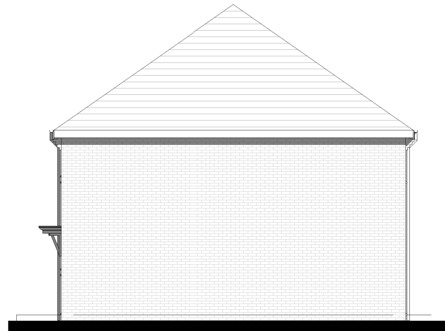
2 Gable 1 1 : 100 Applies to plots 128 & 129
