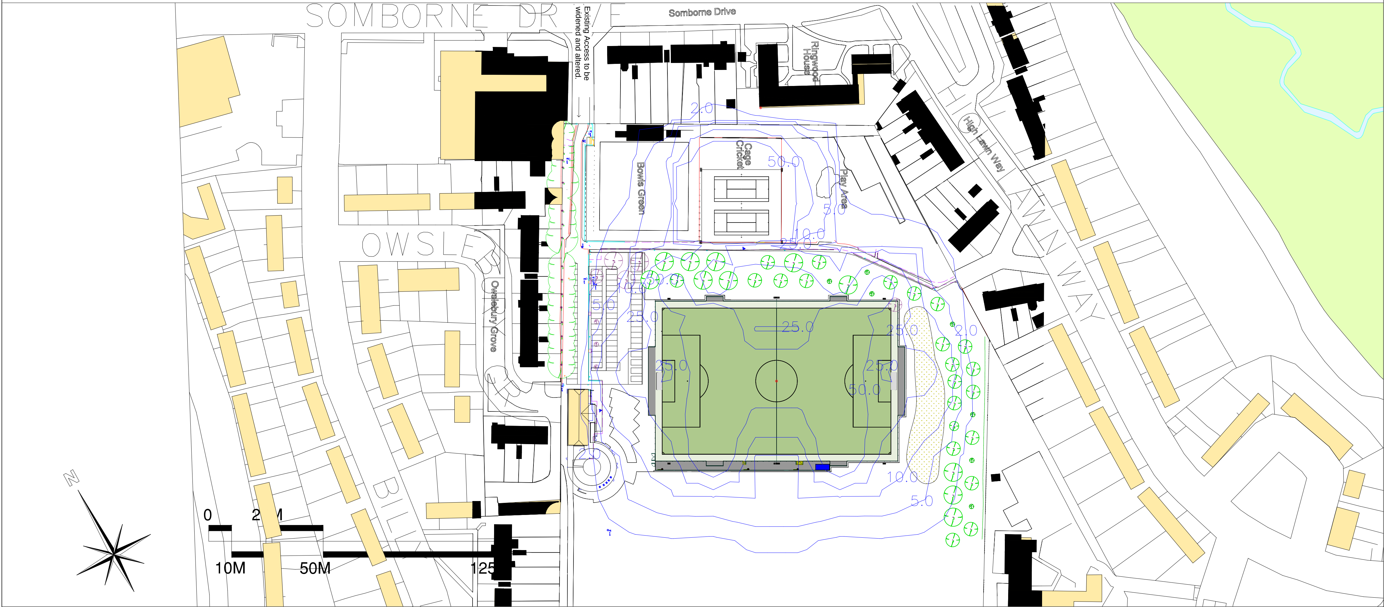
FA Competitive Full Sized Football Floodlighting Scheme - Scale 1:1000 Vertical Illuminance and Spillage at 1.75m Height
