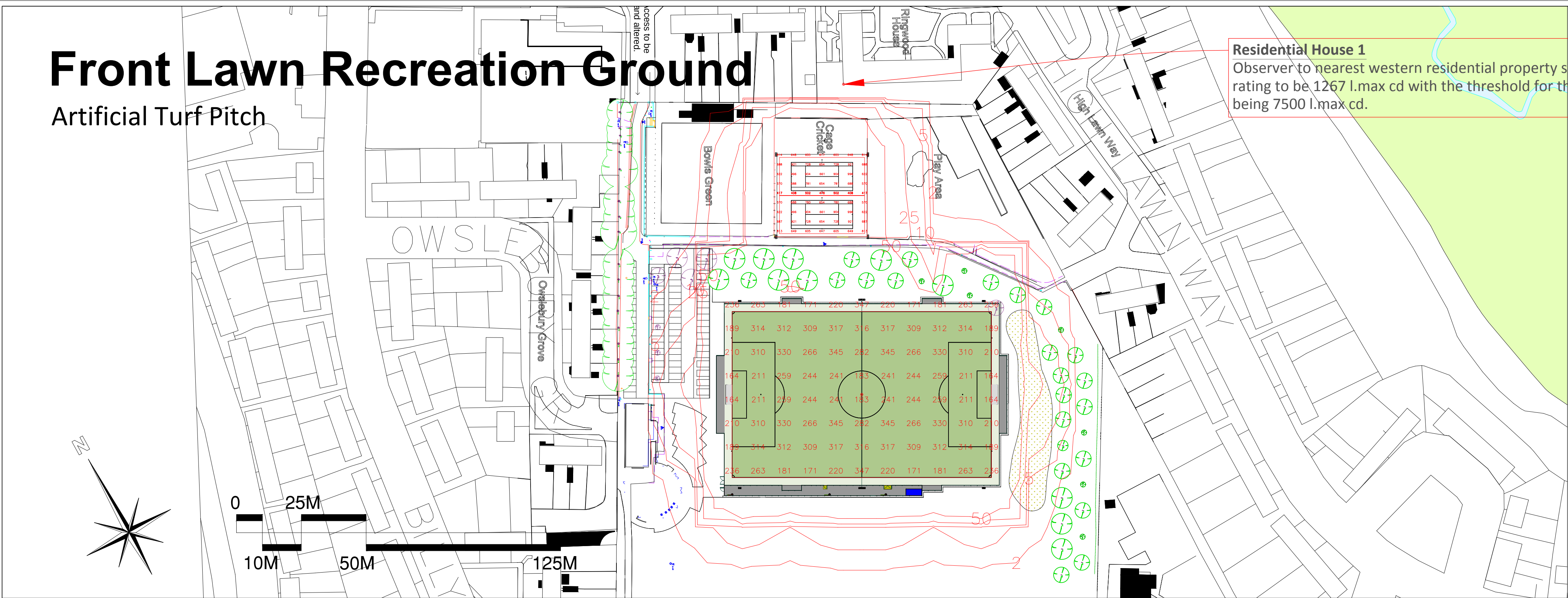
FA Competitive Full Sized Football Floodlighting Scheme - Scale 1:1000 Horizontal Illuminance and Spillage
