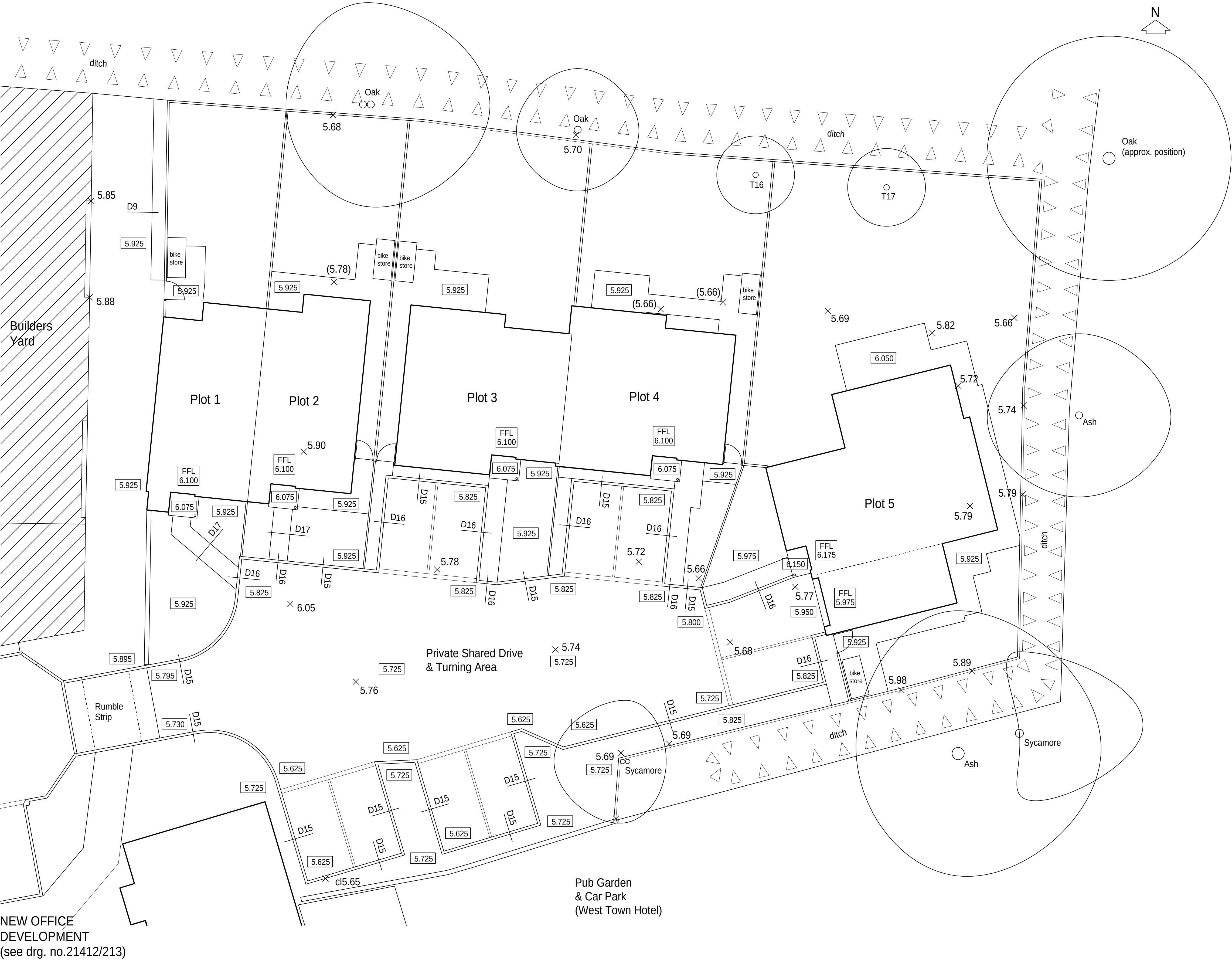
Proposed Hard Landscaping Plan - Residential Site 1:100
