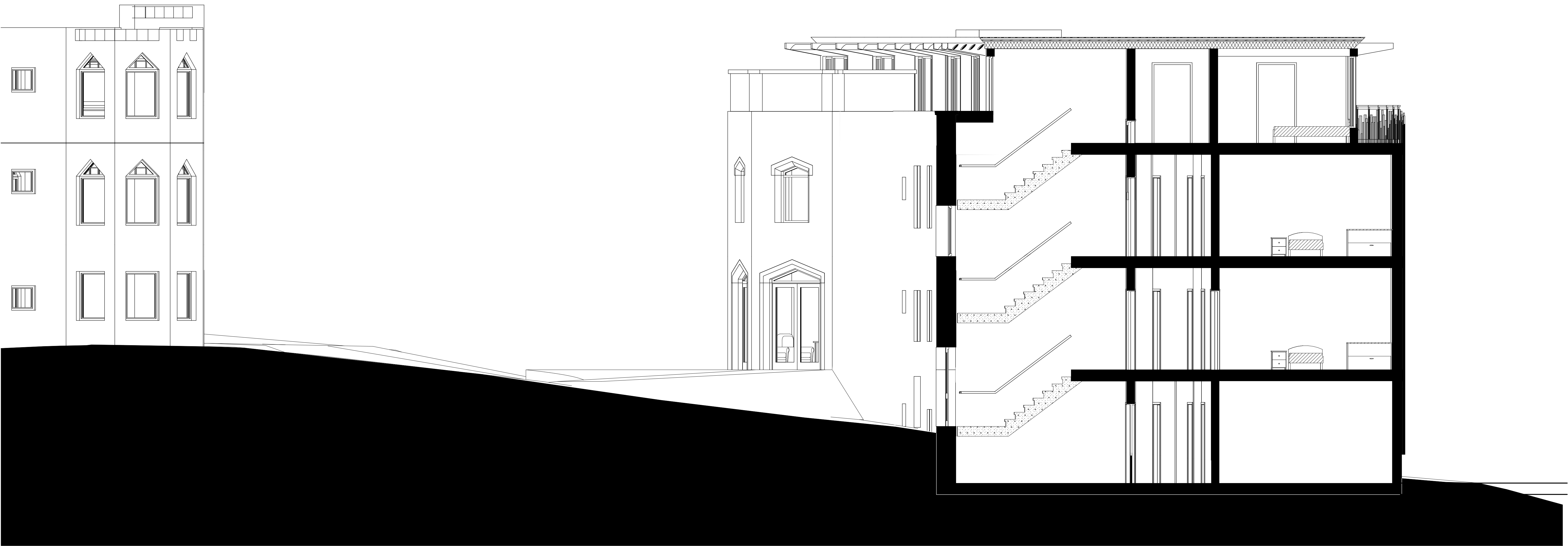
Section B-B
