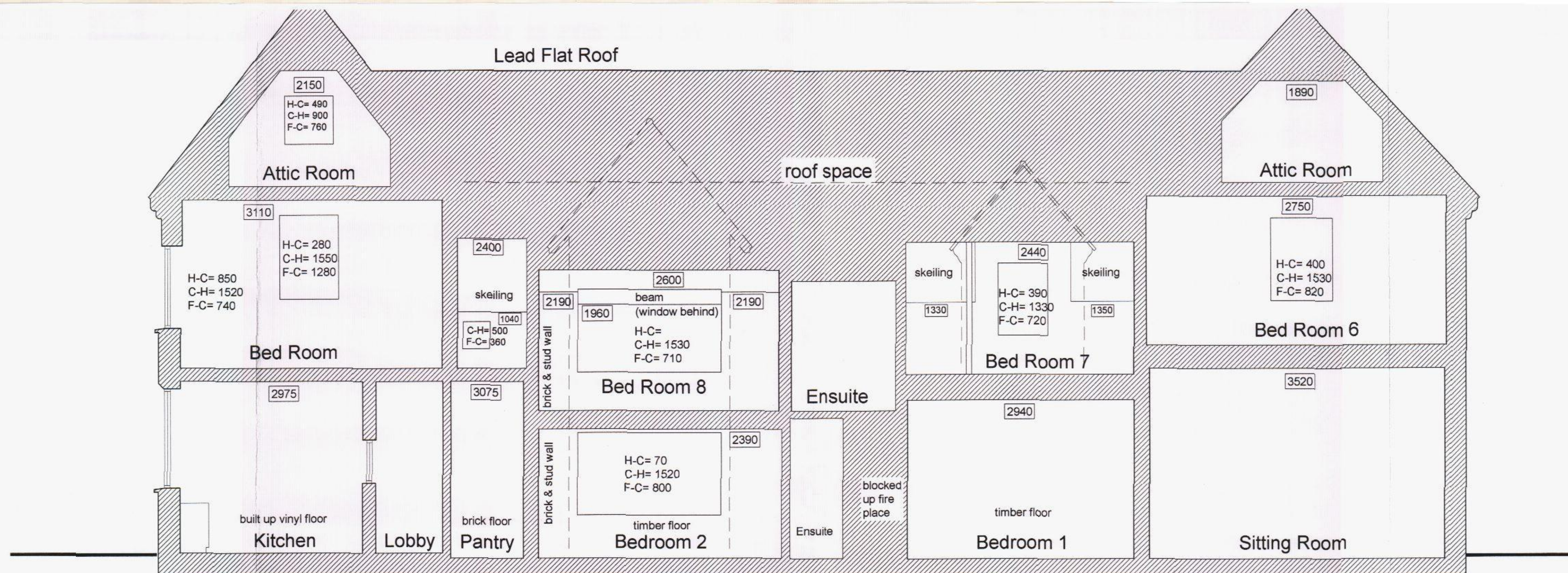
CROSS SECTION CC
