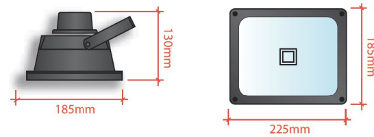
Item 8. Flood light (7 off) 30watt LED flood light with a black case. SCALE 1:10 @ A3
