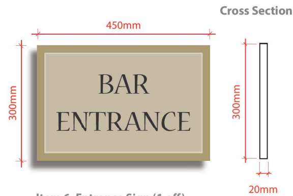
Item 6. Entrance Sign (1 off) Fabricated facility sign. SCALE 1:10 @ A3 AGL:1230mm
