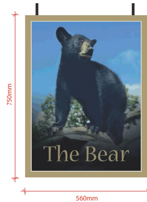
Item 9. Pictorial Sign (1 off) Fabricated double-sided hanging pictorial sign, complete with applied digital prints. To be fitted to the existing gibbet.
