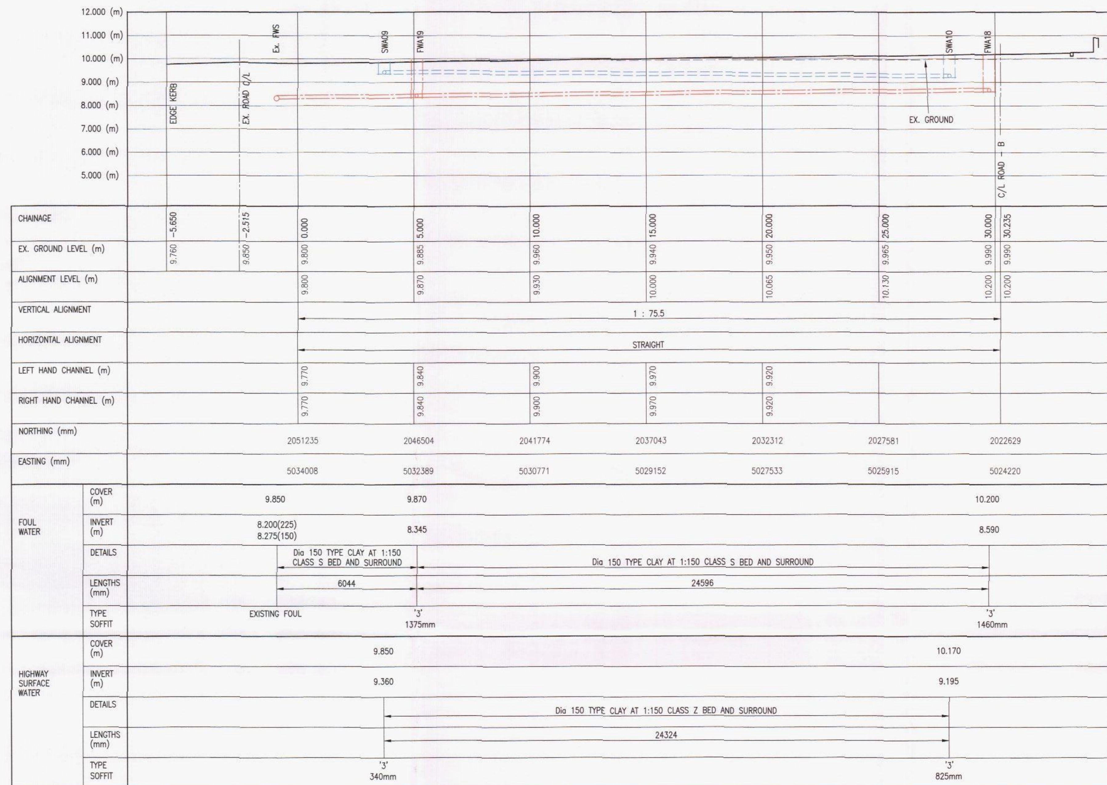
ACCESS ROAD - A - LONG SECTION (HORIZONTAL SCALE 1:100 - VERTICAL SCALE 1:100)
