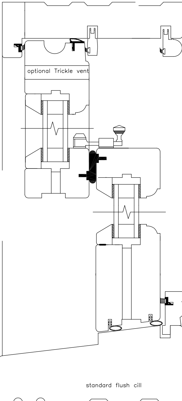
Section A-A Conservation Sash Window - Head & Cill
