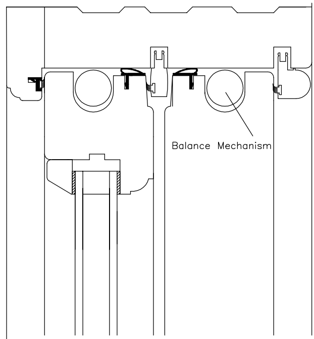
Section B Conservation Sash Window Jamb
