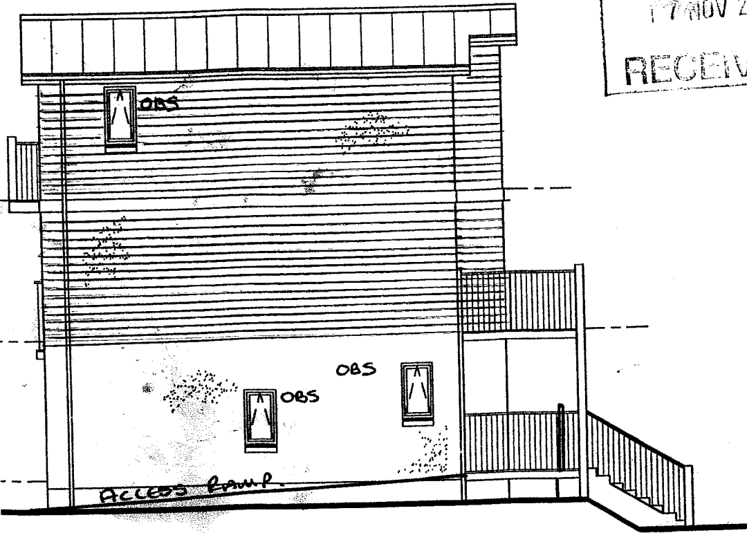
Side Elevation
