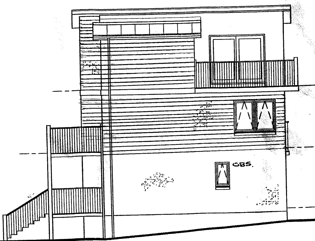
Side Elevation
