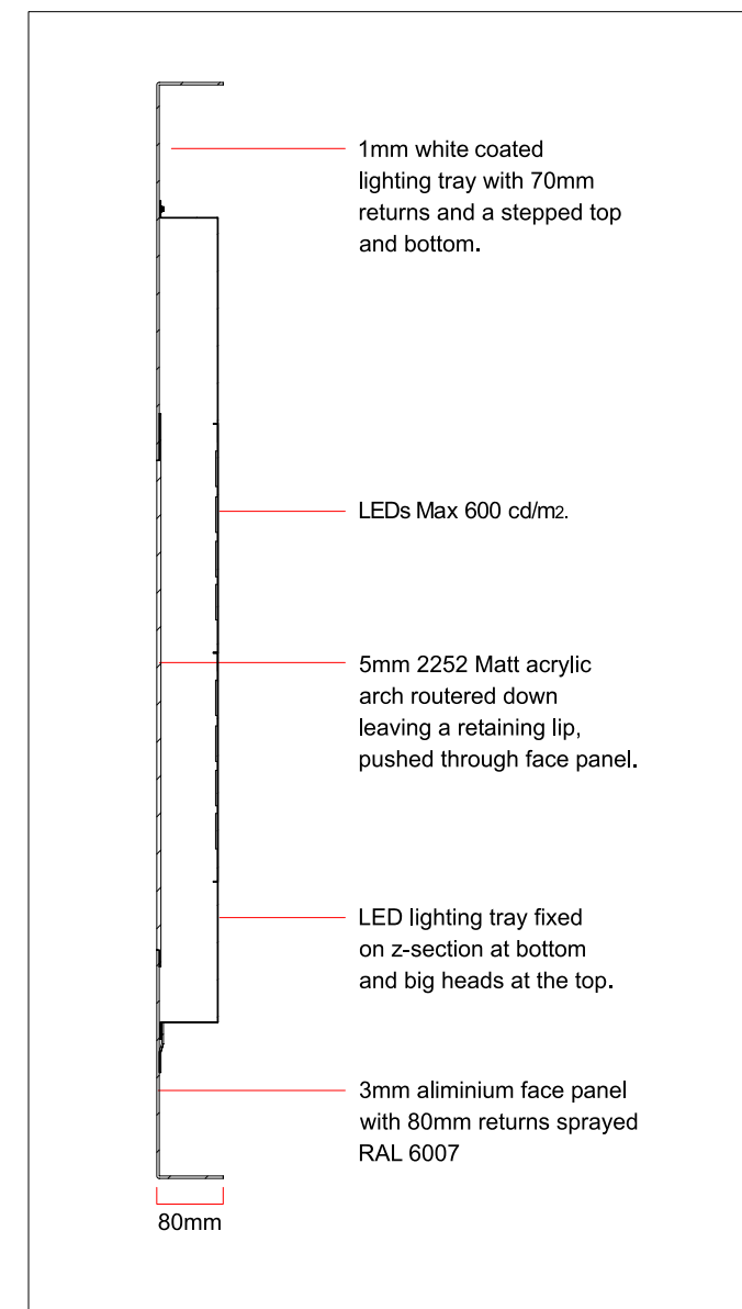
Letters Section scale 1:10
