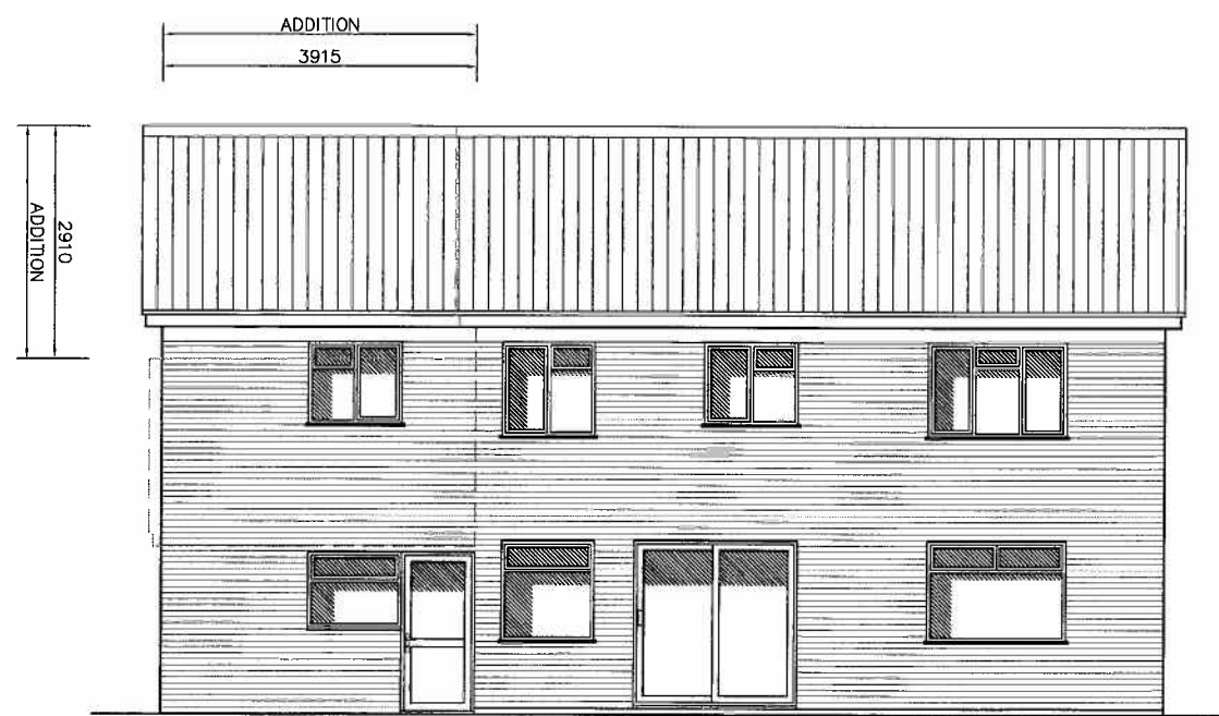
SOUTH
