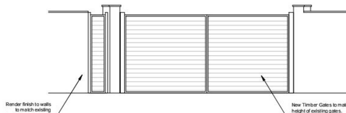
Elevation on Proposed Timber Gates
