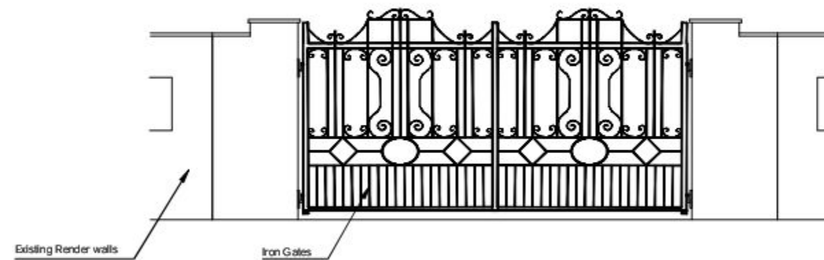
Elevation on Existing Iron Gates
