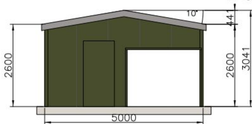
Front Elevation (External)
