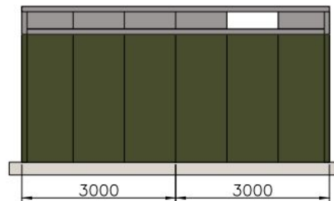
Left Elevation (Scale = 1:75)
