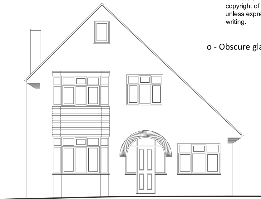
NORTH ELEVATION
