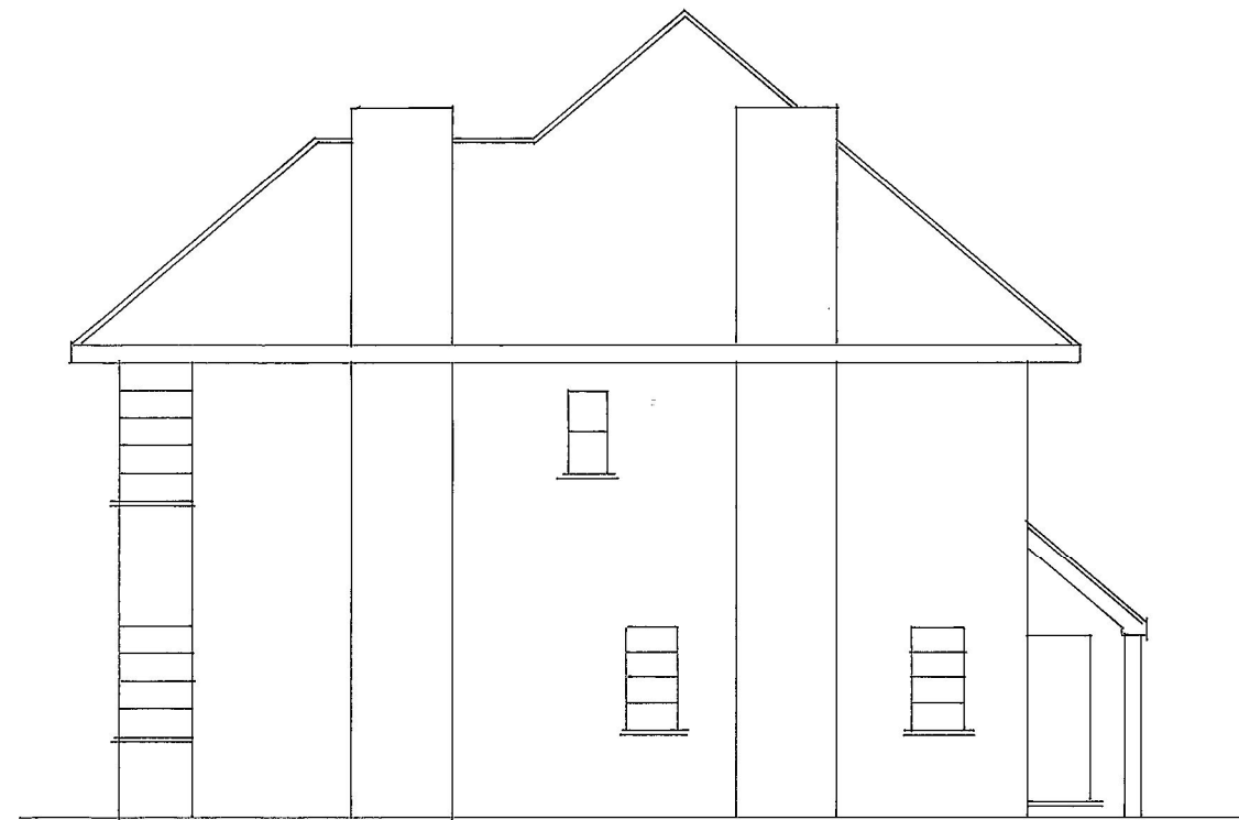
Existing South/Side Elevation
