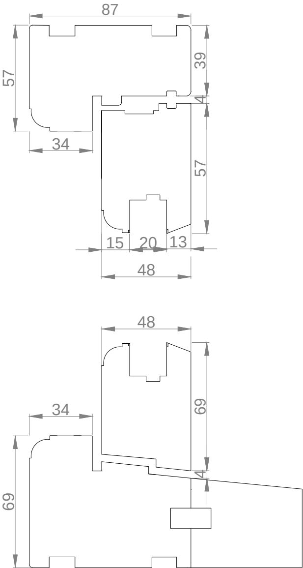
Drawing 014 - Proposed Casement Window - Section - SCALE: 1:2
