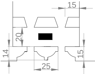
Drawing 013 - Propose Glazing Bar - Section - SCALE: 1:2
