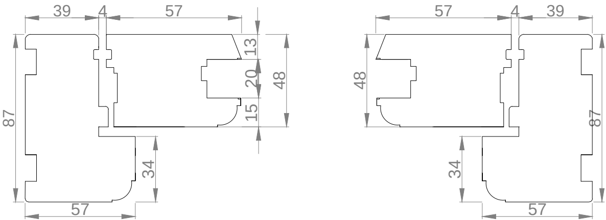
Drawing 012 - Proposed Casement Window - Plan View - Section - SCALE: 1:2
