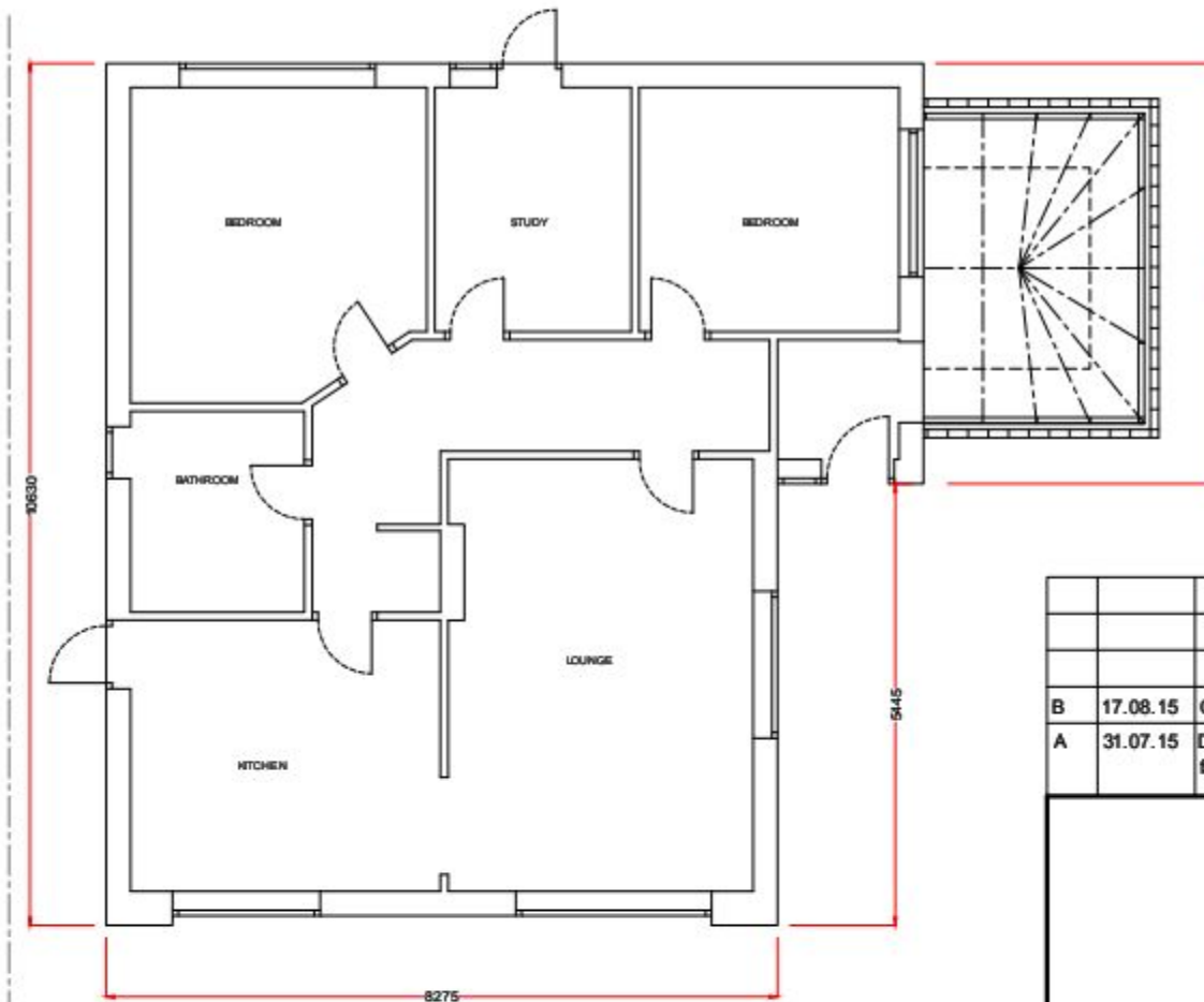
PLAN
