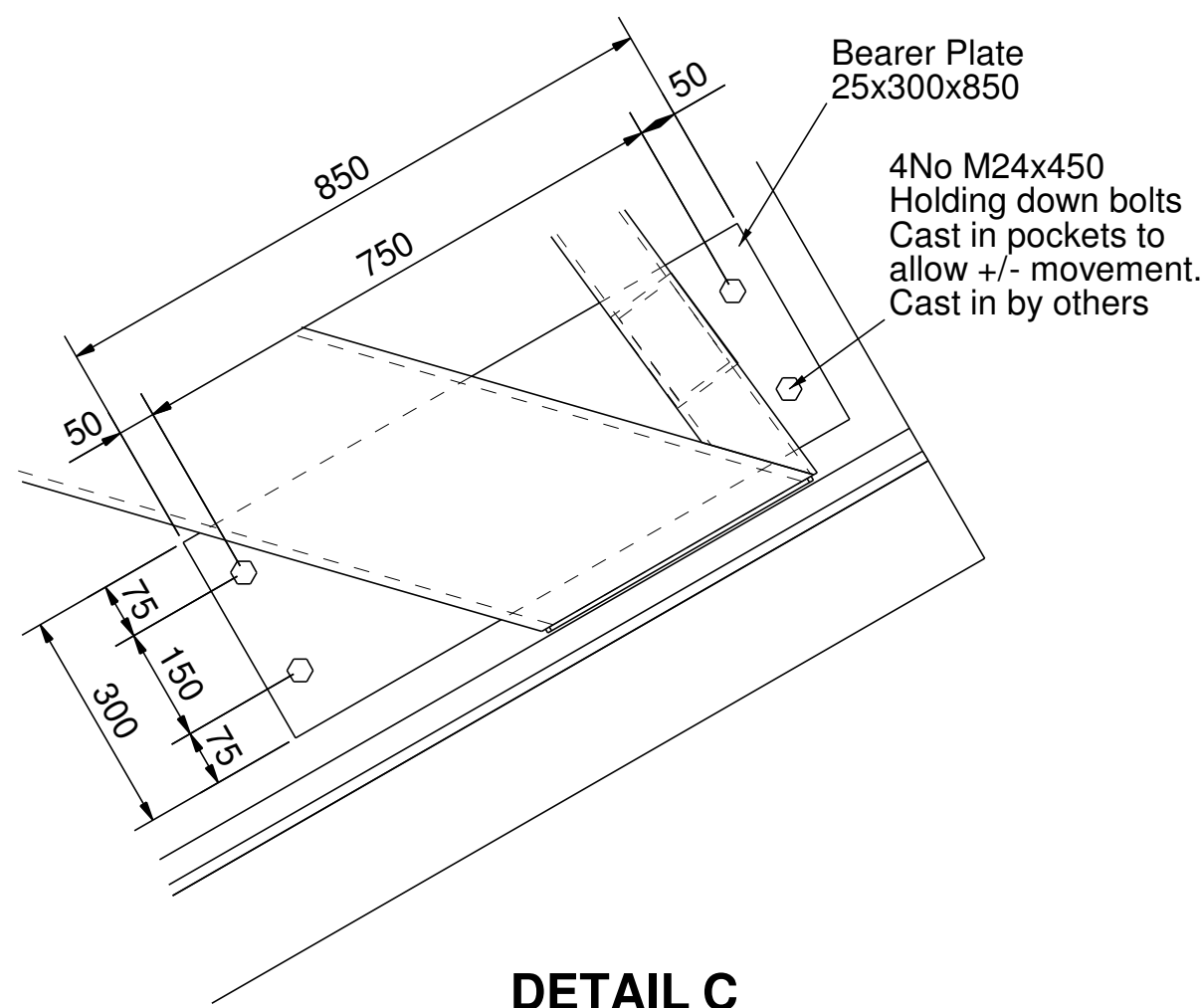
DETAIL C TAKEN FROM DRAWING 06
