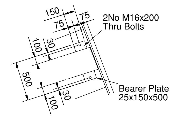
DETAIL D 1:25
