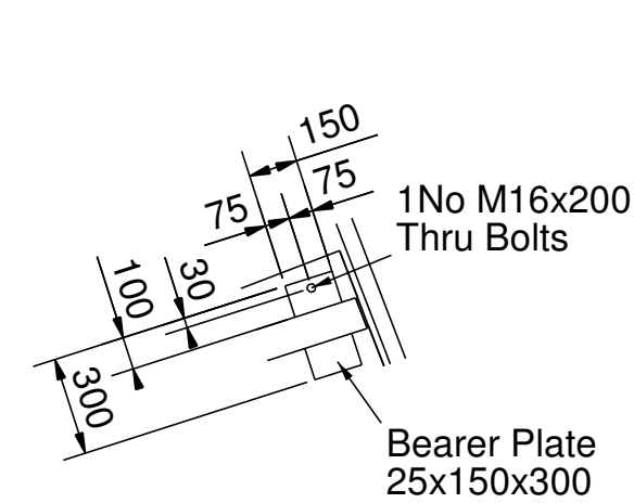
DETAIL C 1:25
