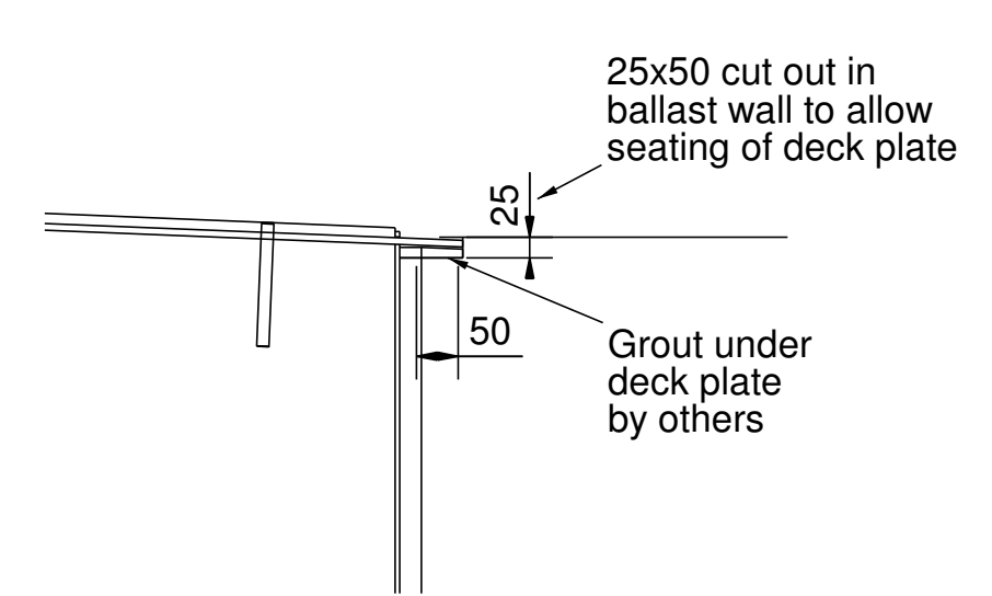
C - C TAKEN FROM DRAWING 02
