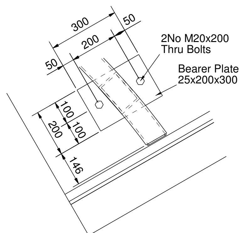
DETAIL B TAKEN FROM DRAWING 06
