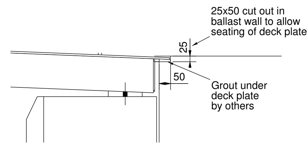
B - B TAKEN FROM DRAWING 02
