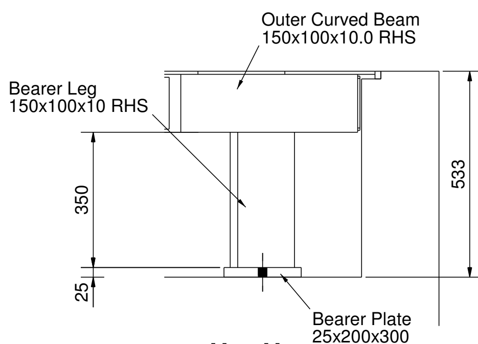
H - H TAKEN FROM DRAWING 06
