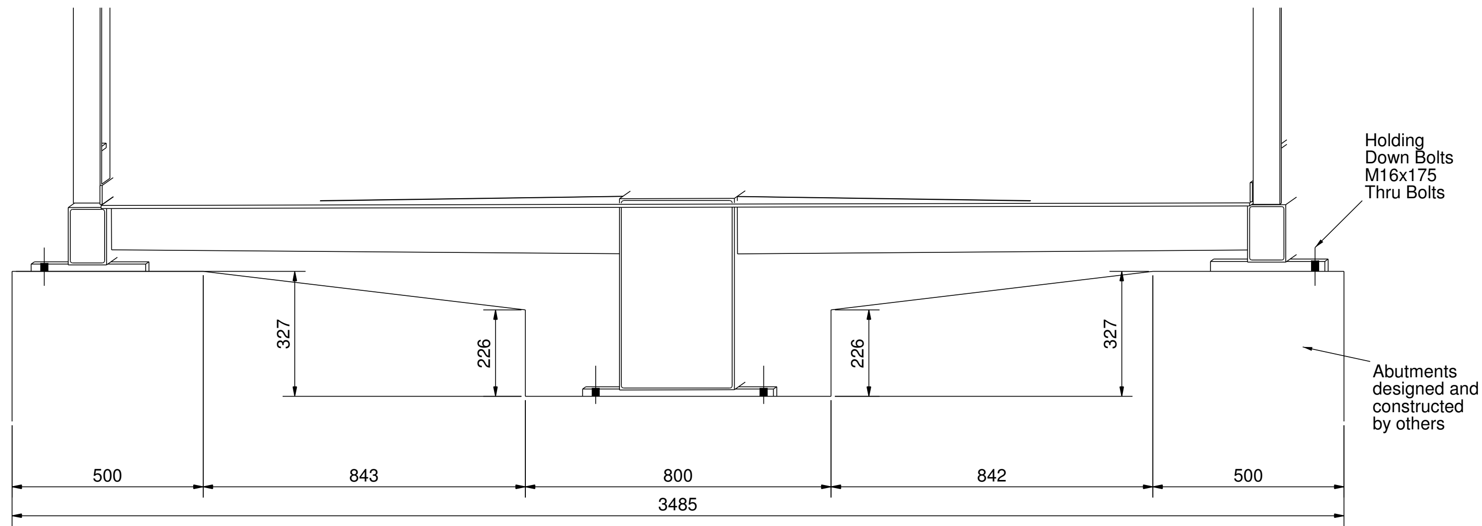
A - A TAKEN FROM DRAWING 02
