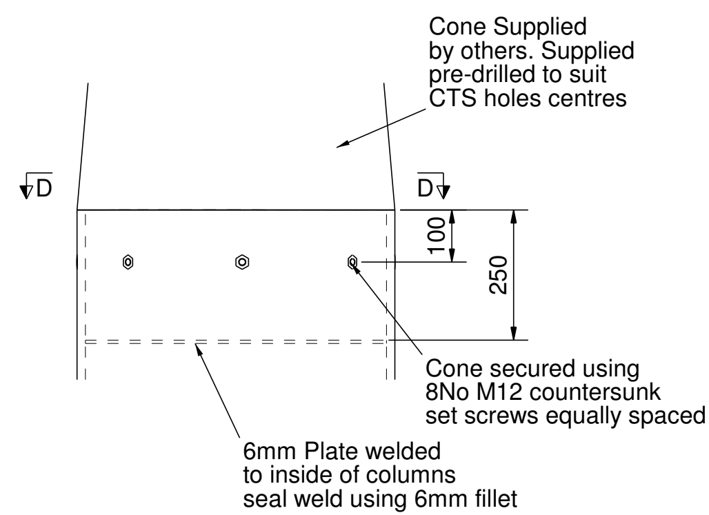
TOP OF COLUMN 1:10
