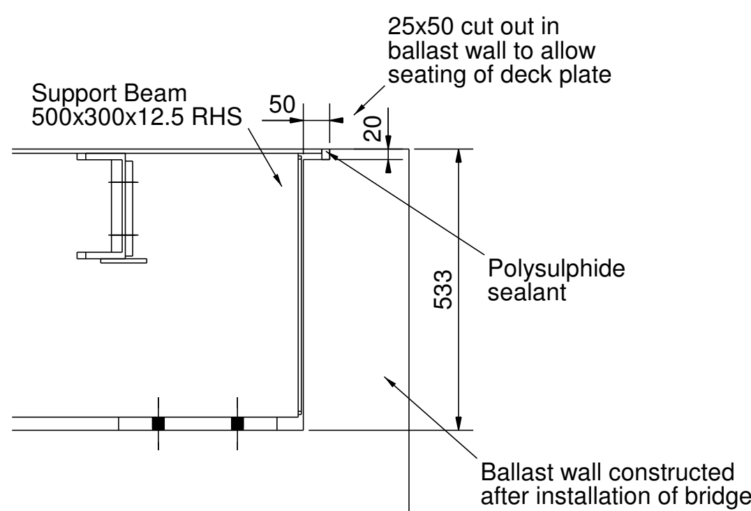
I - I TAKEN FROM DRAWING 06
