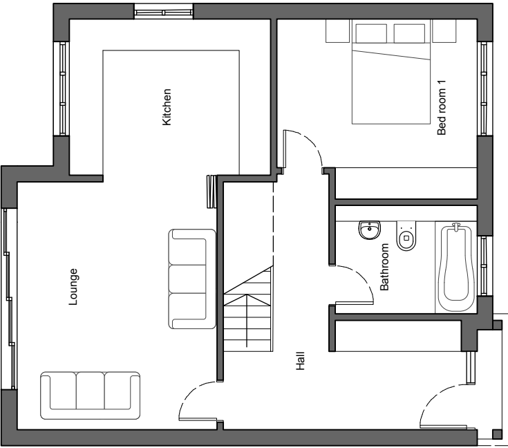
Ground floor plan Area = 66m2
