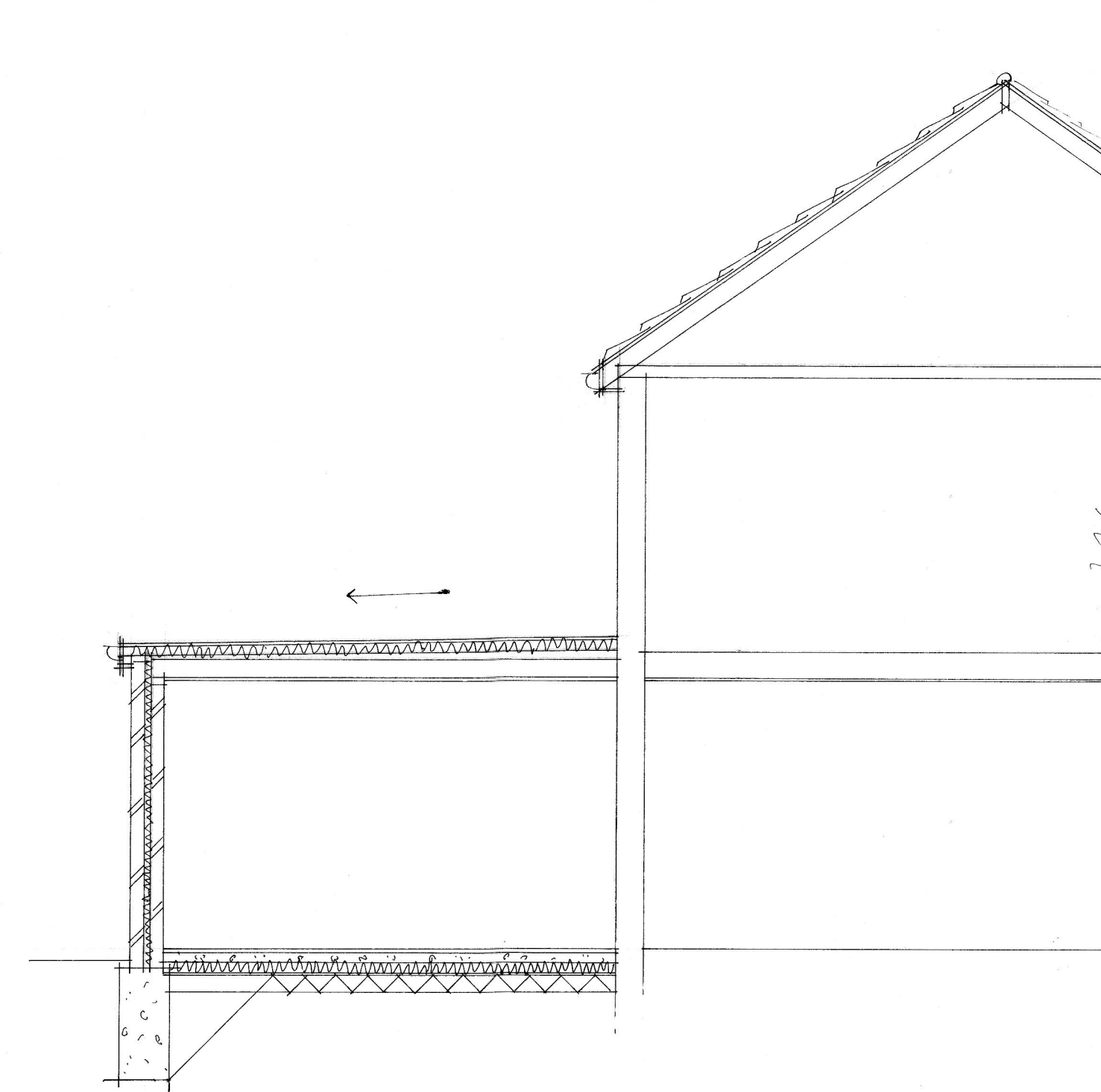
section a.a.
