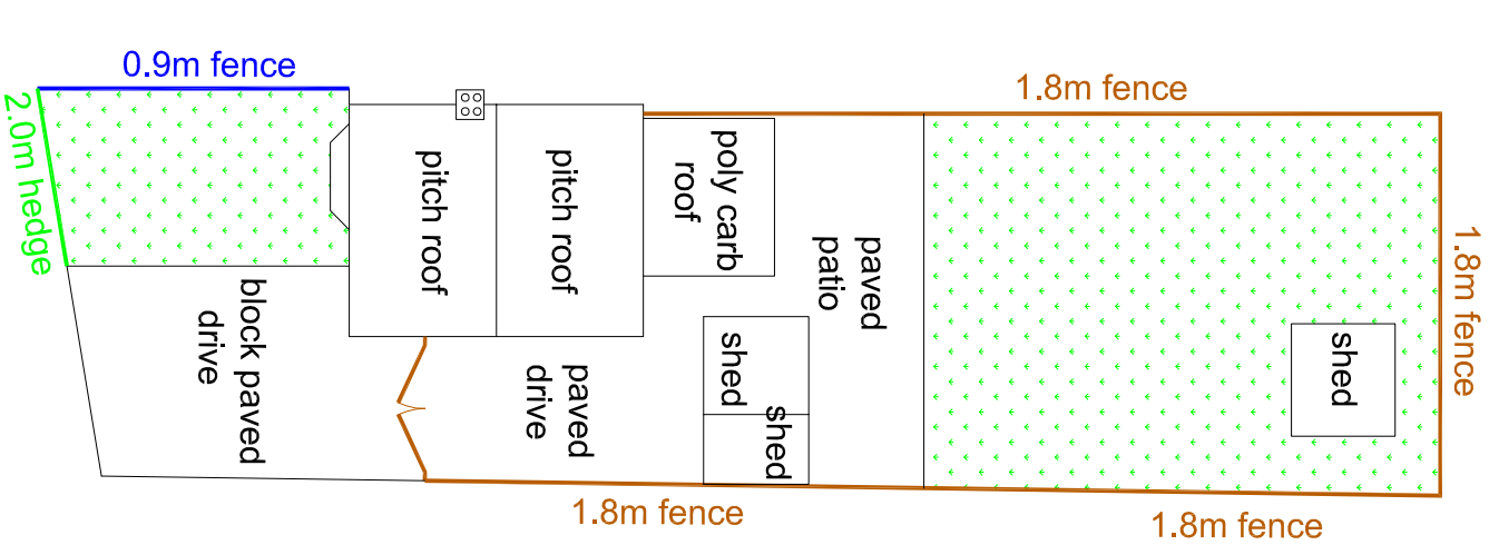
EXISTING BLOCK PLAN SCALE 1:200
