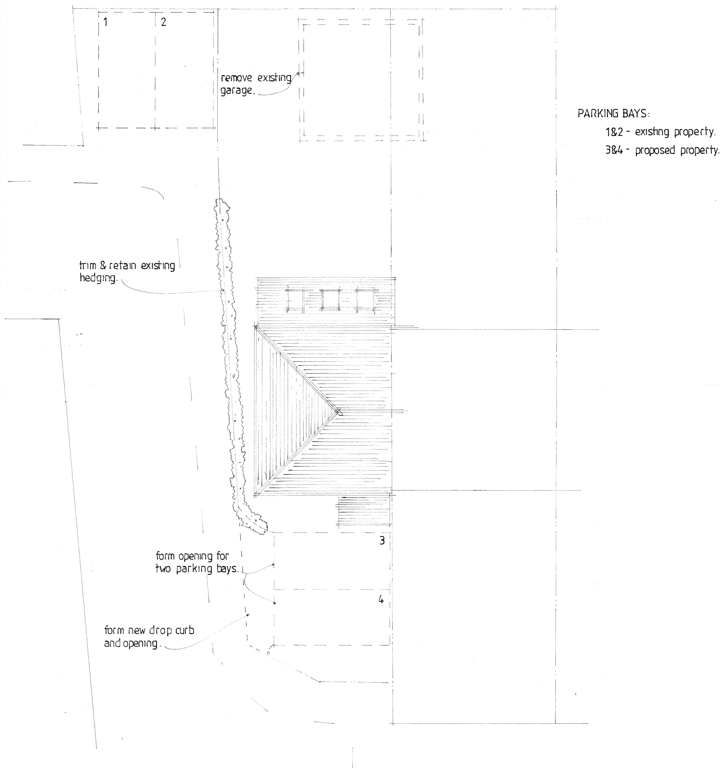
PROPOSED SITE LAYOUT. 1:100
