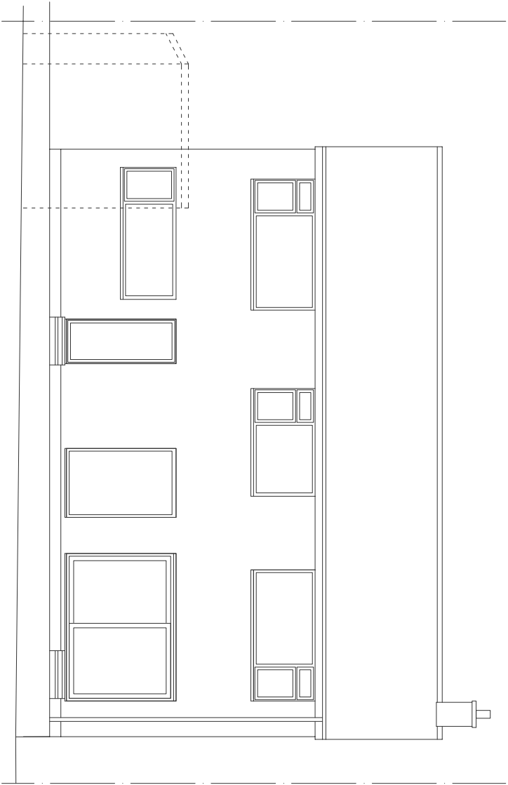
Existing South
