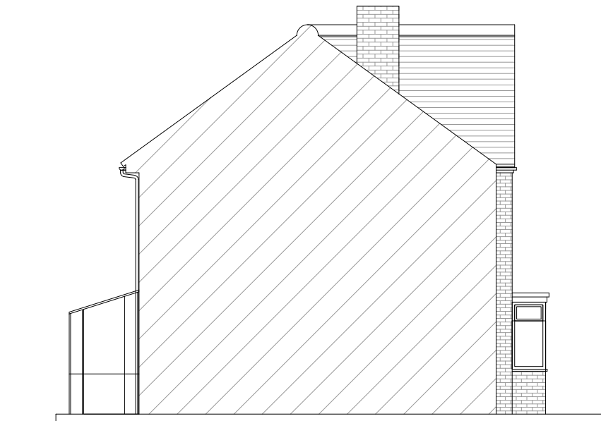
Existing Side Elevation/Section
