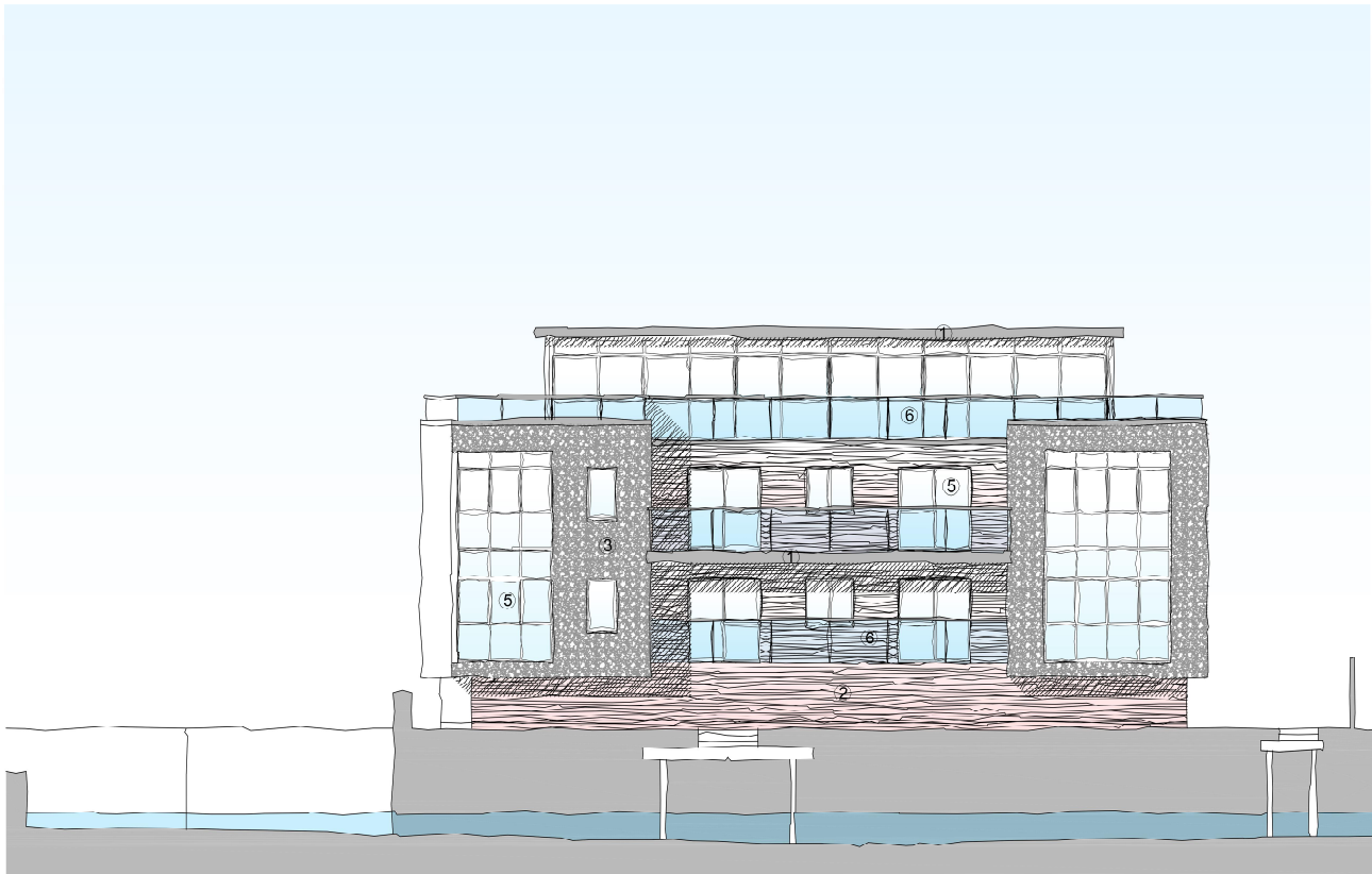
South Elevation
