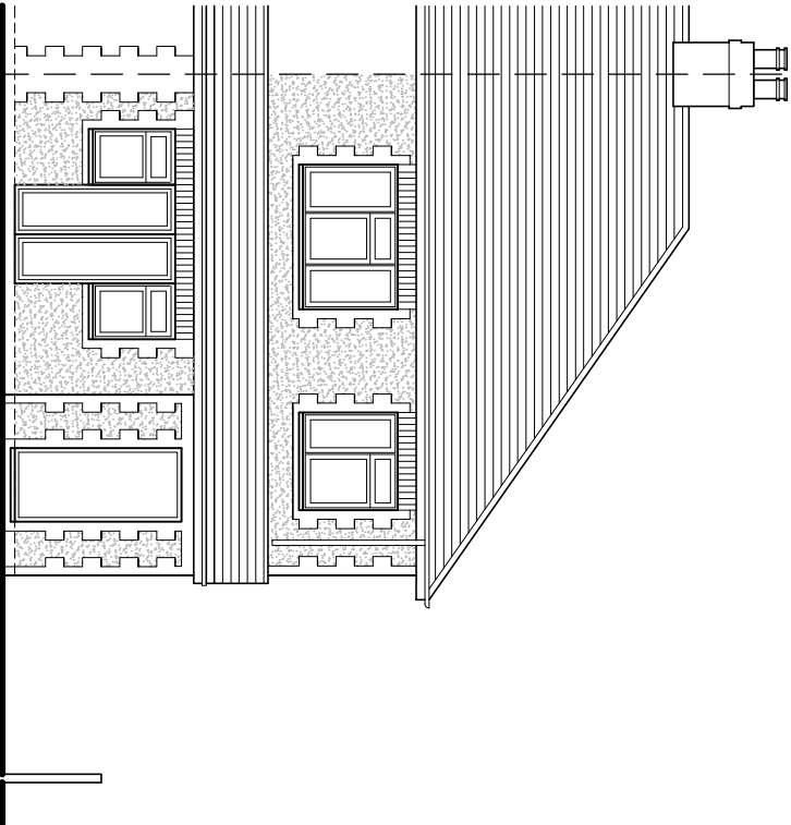
no.14 | no.16 South (front) elevation
