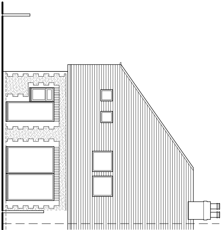
North (rear) elevation
