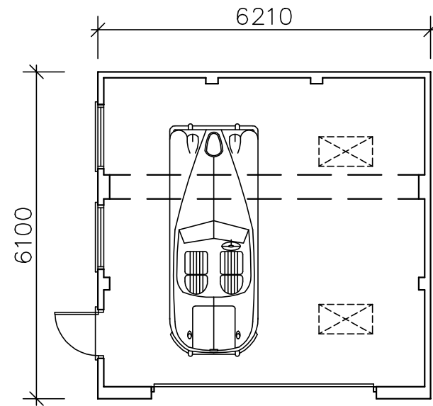
FLOOR PLAN
