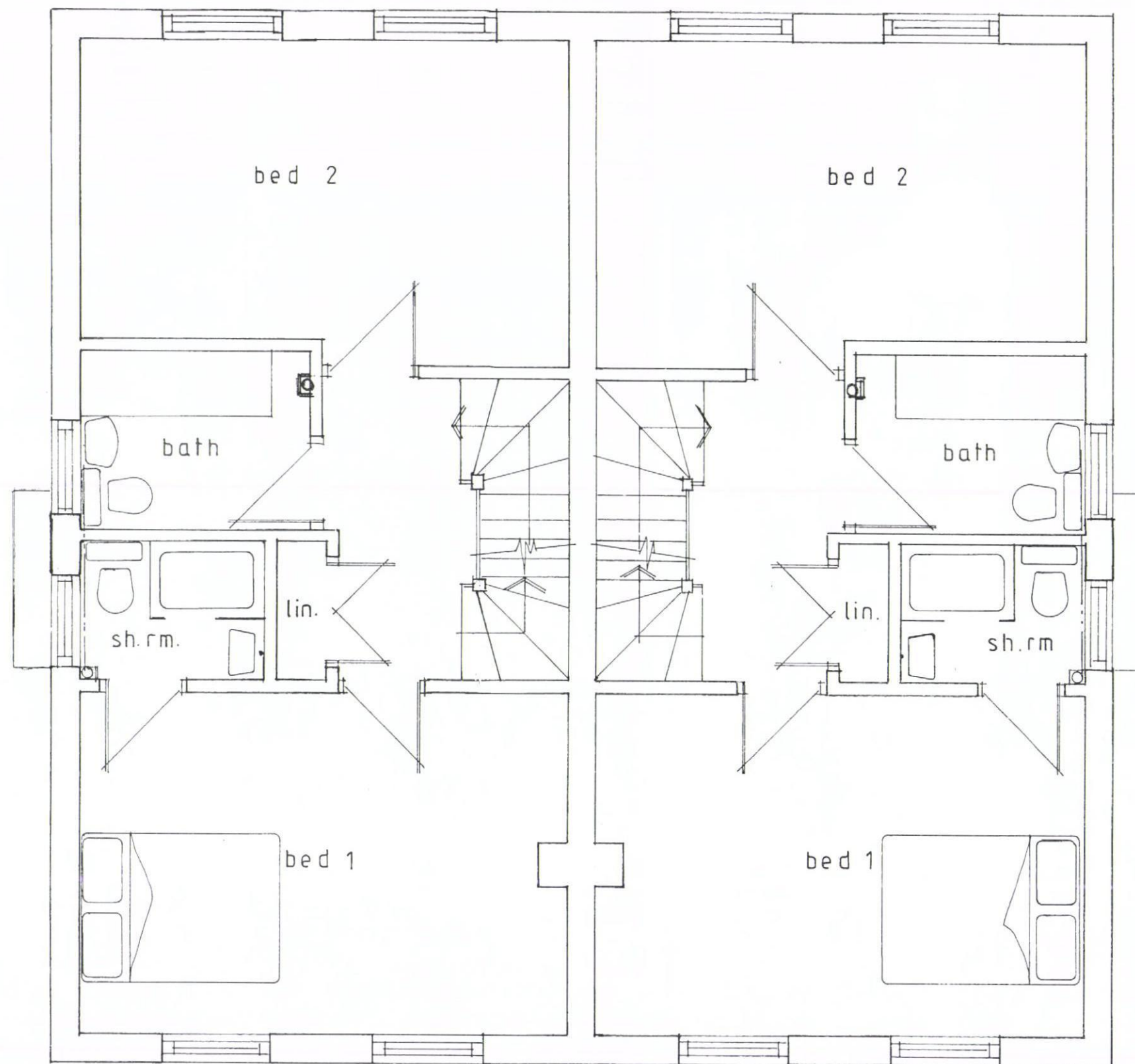
FIRST FLOOR 1:50
