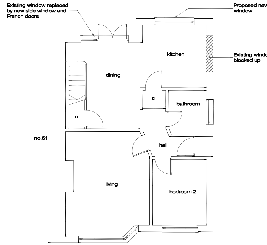
Ground Floor Plan - As Proposed
