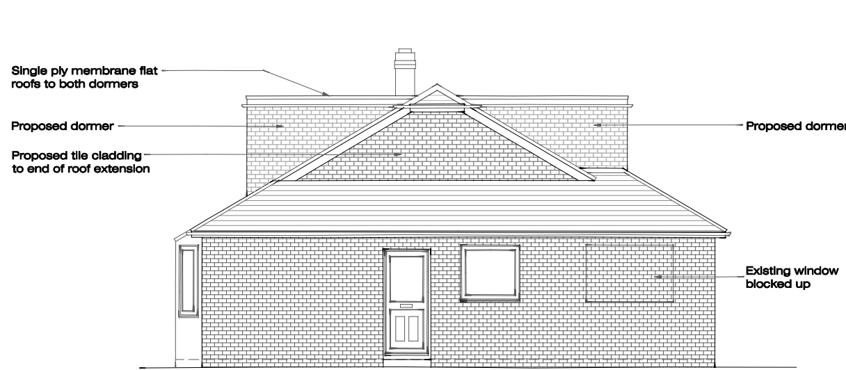
South-East (Side) Elevation - As Proposed
