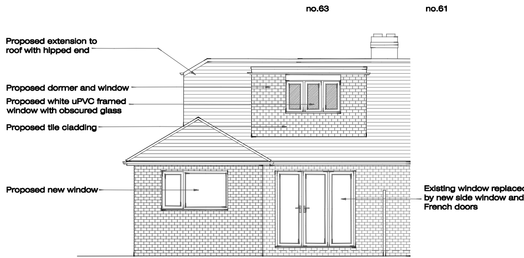
North-East (Rear) Elevation - As Proposed
