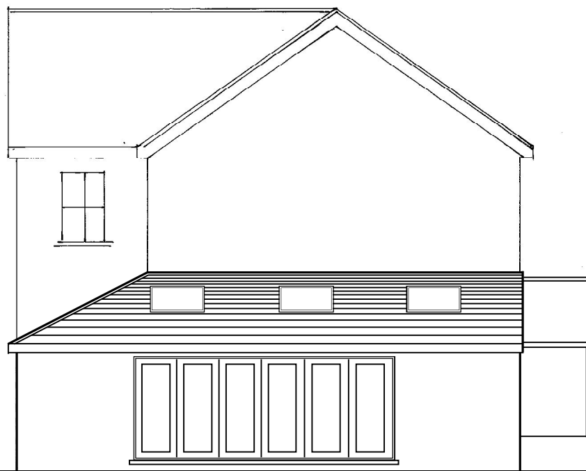
Proposed North/Side Elevation
