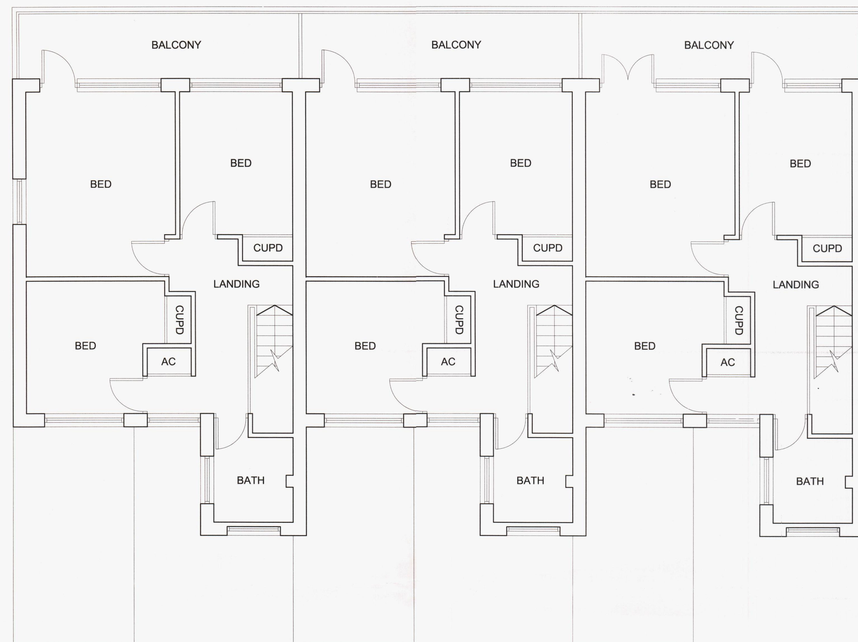
EXISTING FIRST FLOOR 1-50
